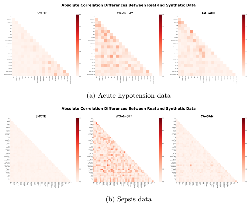
Fig. A: Absolute difference in correlations between real data and the synthetic data generated with SMOTE, WGAN-GP*, and CA-GAN.
