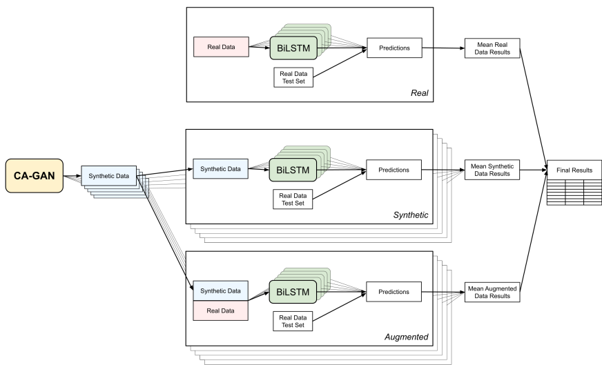
Fig. A: Diagram of BiLSTM Model Training for Continuous Variable Prediction.
