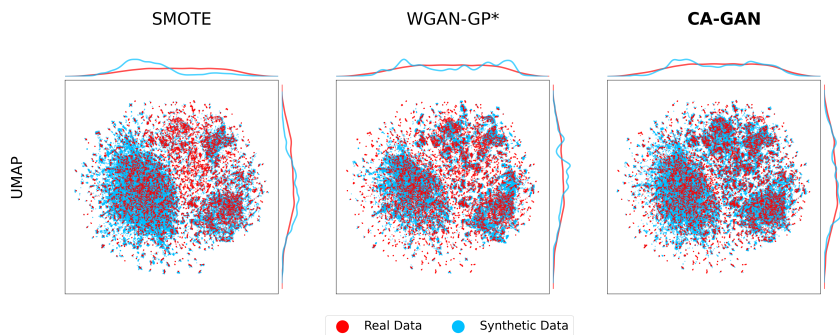
Fig. A: UMAP two-dimensional representations of the acute hypotension dataset for Black patients.
