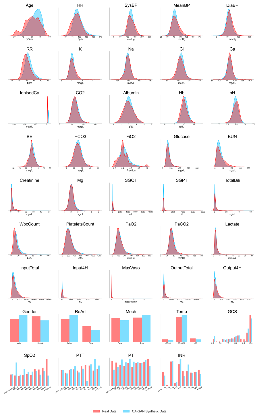
Fig. A: Overlaid distribution plots of real data and CA-GAN synthetic data for each variable in the sepsis dataset.
