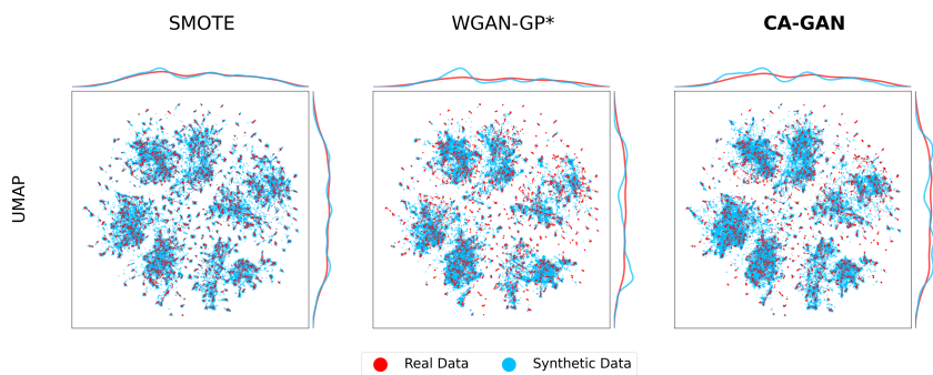
Fig. B: UMAP two-dimensional representations of the sepsis dataset for Black patients.
