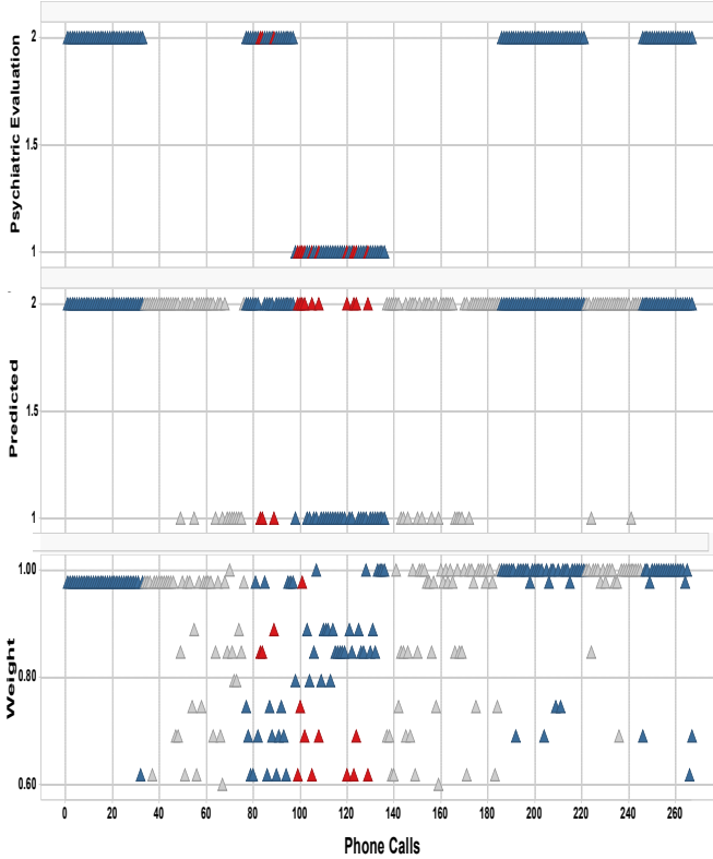
Figure 5: Results from the induced model of patient P0702 and the assessments from the psychiatrist.
