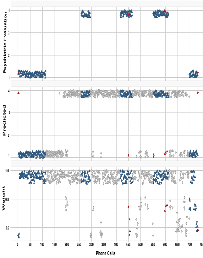
Figure 4: Results from the induced model of patient P0201 and the assessments from the psychiatrist.
