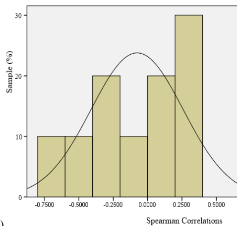
Fig. 1. Distributions of Spearman correlations between an amount of speech activity and a) PA and b) NA
